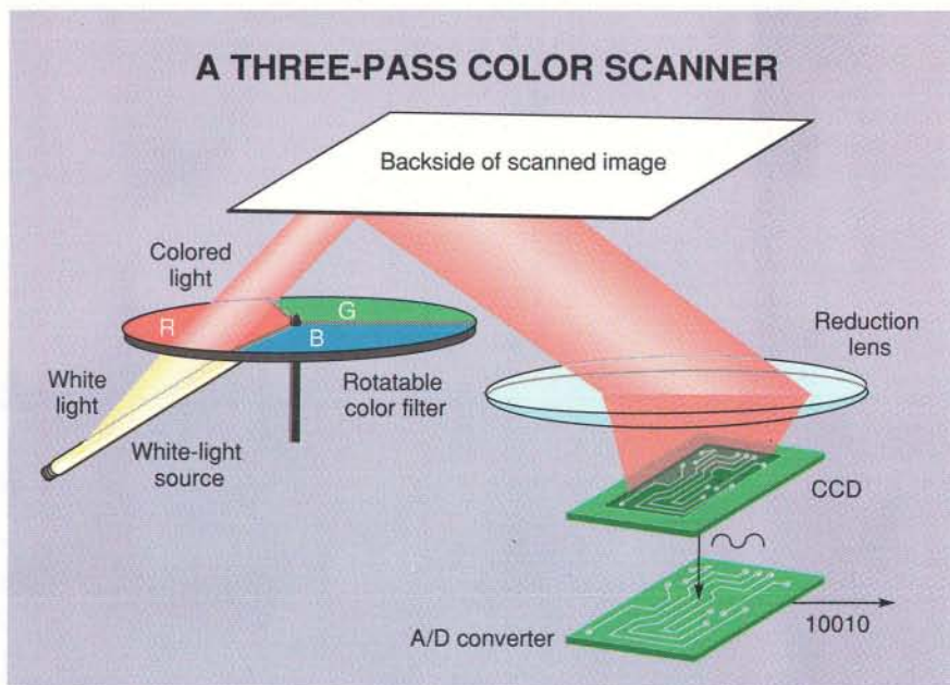
Figure 2: For each scan line, a white-light source shines through red, green, and blue filters.
